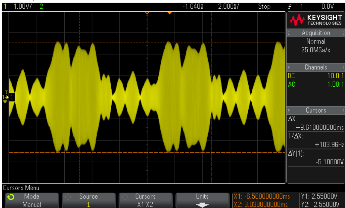
Figure 9b: 100W PEP speech envelope, \approx 6 dB compression.
